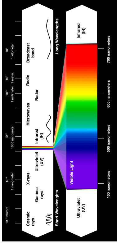
Figure 4.1: The Electromagnetic Spectrum
